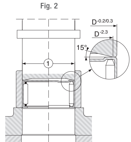
(1) Bore of ring D + 0.3 mm
