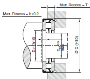
Mounting for high speed rotation
