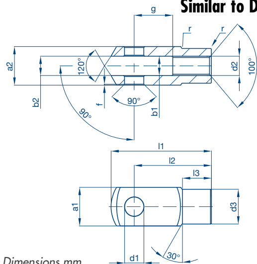
Dimensions mm
