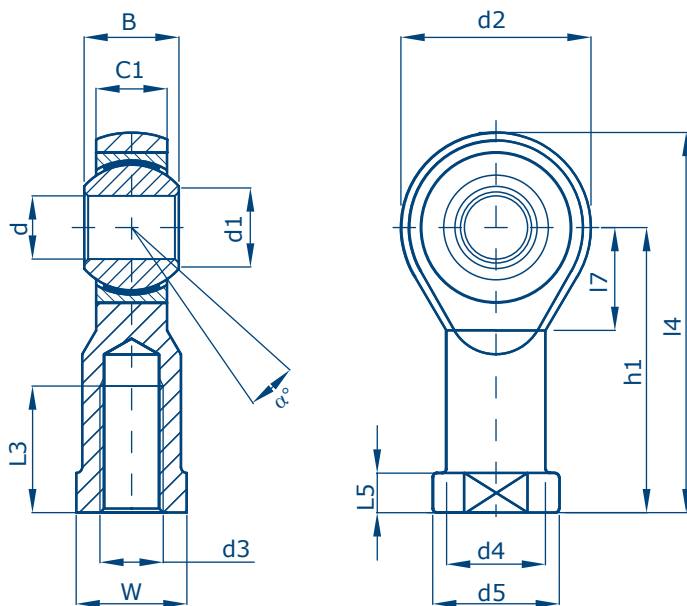
Dimensions mm
