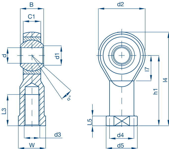
Dimensions mm
